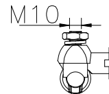
LV BUSHING TERMINAL DETAIL
